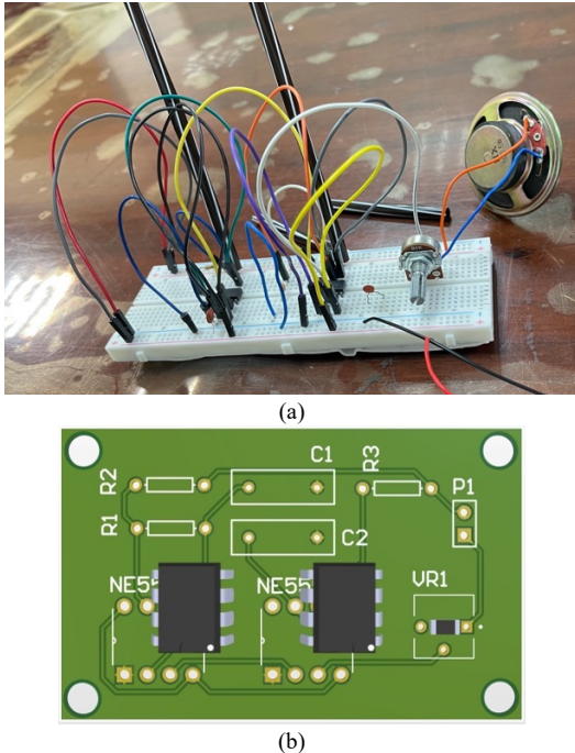
Fig. 2. (a) A test set and (b) work-in-progress circuit board for the portable Theremin.
